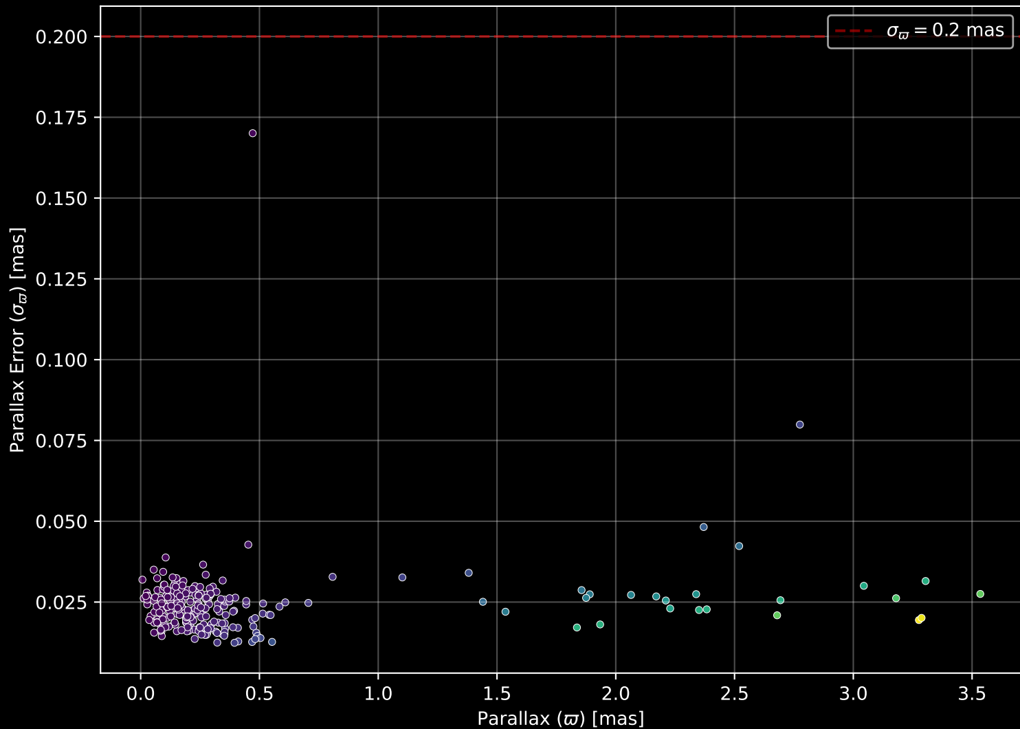
APOGEE DR17 Field: [335-12] Parallax Quality (n= 254)
