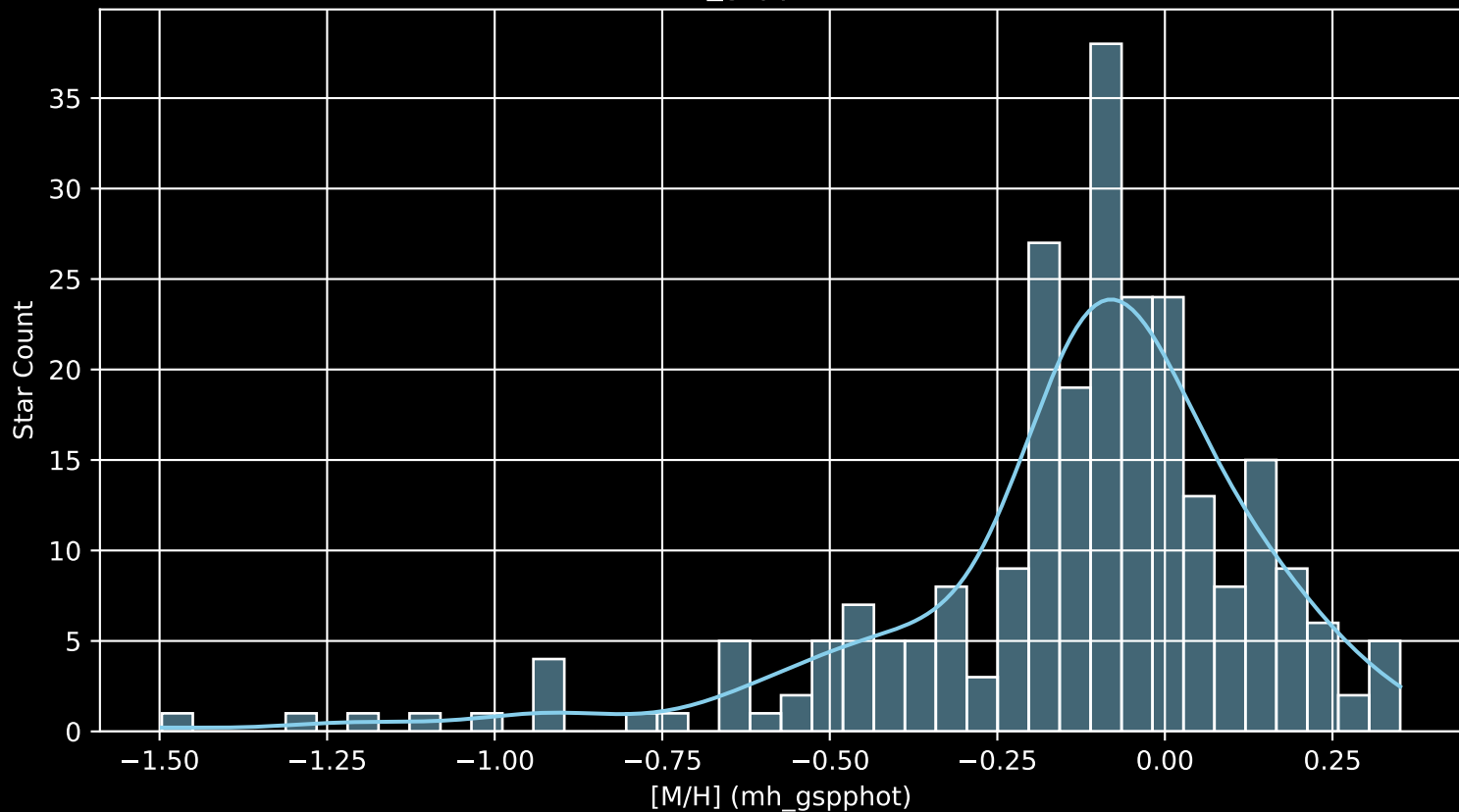
APOGEE DR17 Field: [335-12 [M/H] (mh_gspphot) (n= 251)
