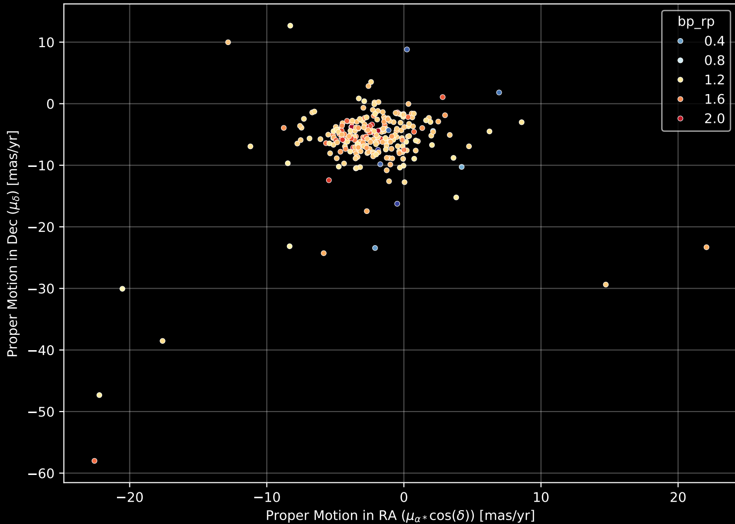
APOGEE DR17 Field: [335-12] Proper Motion Diagram (n= 254)
