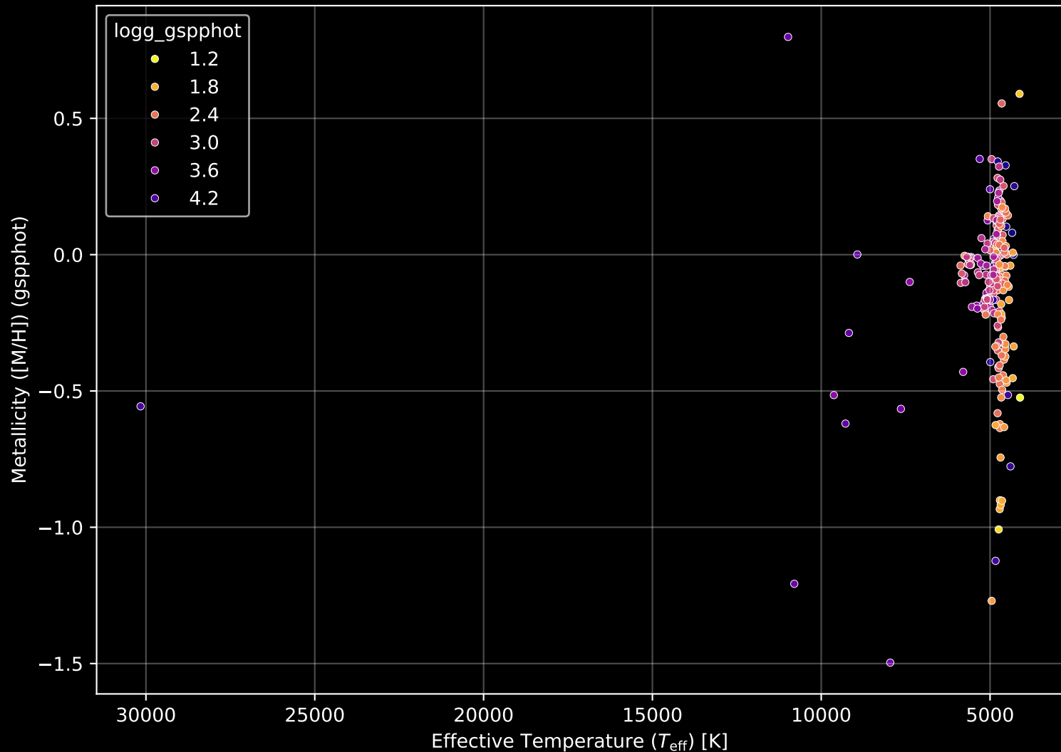
APOGEE DR17 Field: [335-12] Stellar Population Parameters (n= 254)
