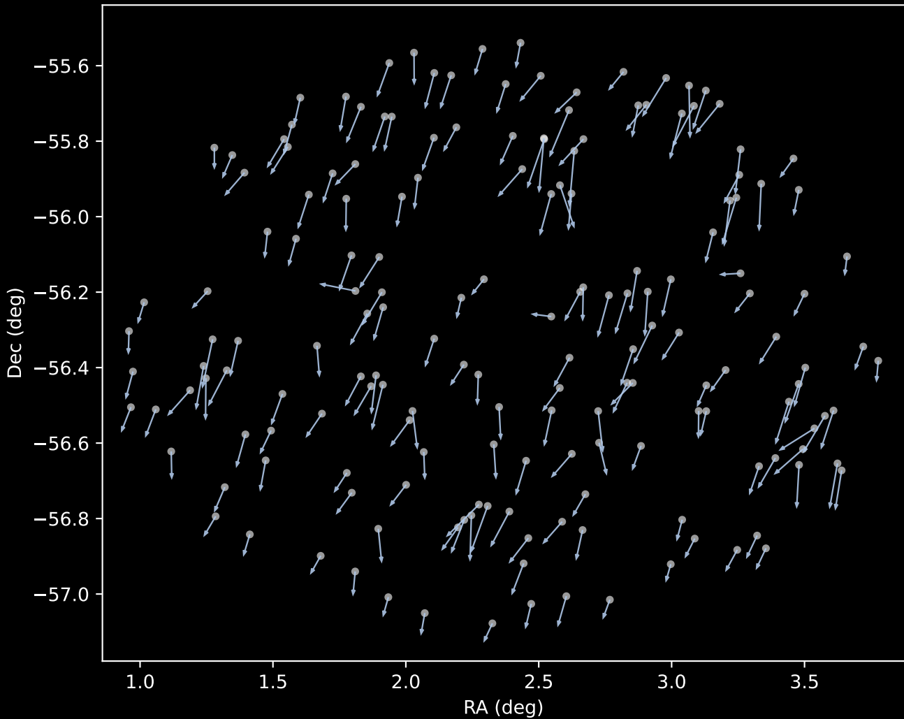
APOGEE DR17 Cluster 1 Proper Motion Vectors (n=172)
