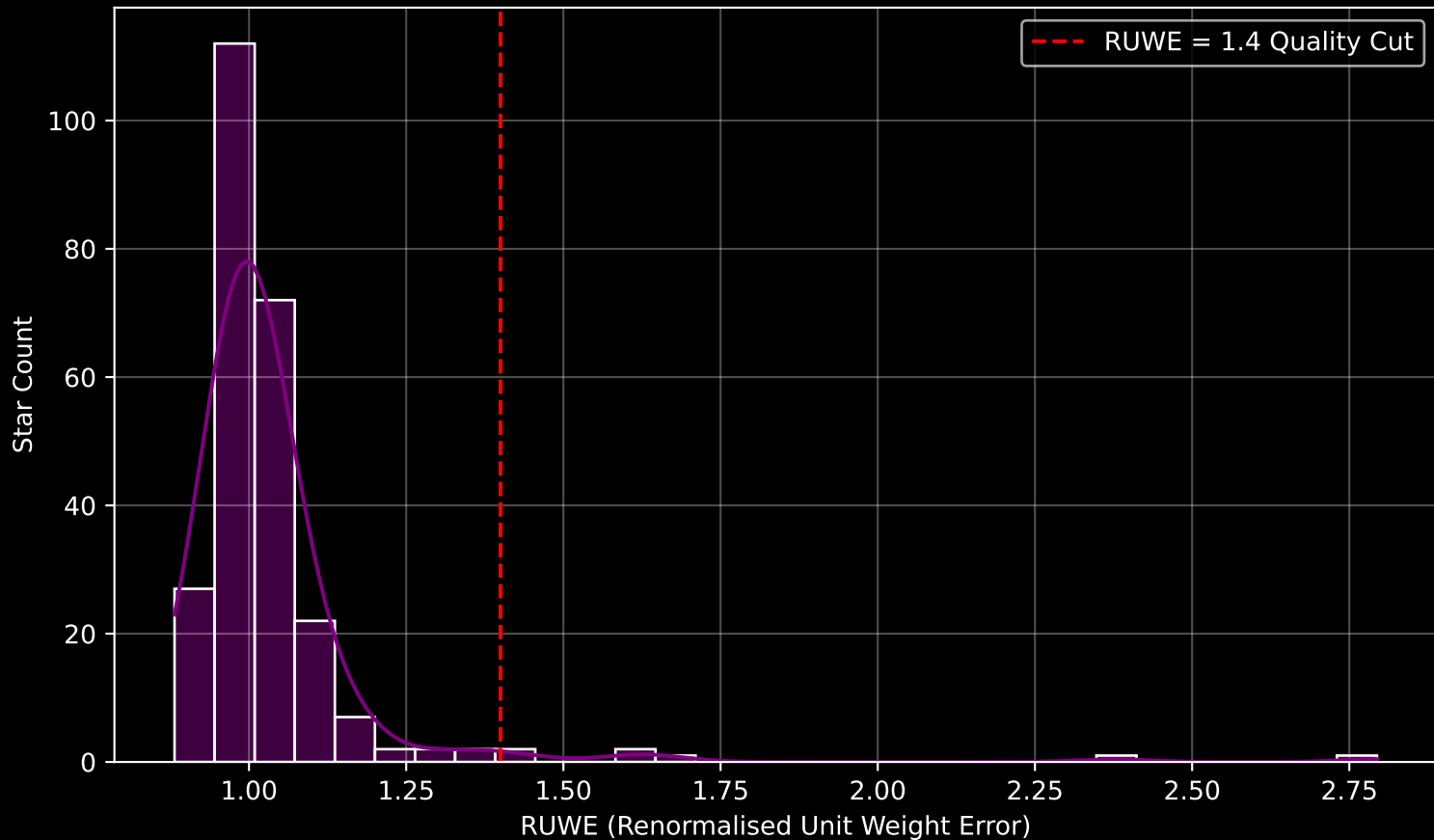
GAPOGEE DR17 Field [335-12] RUWE Distribution (n= 253)
